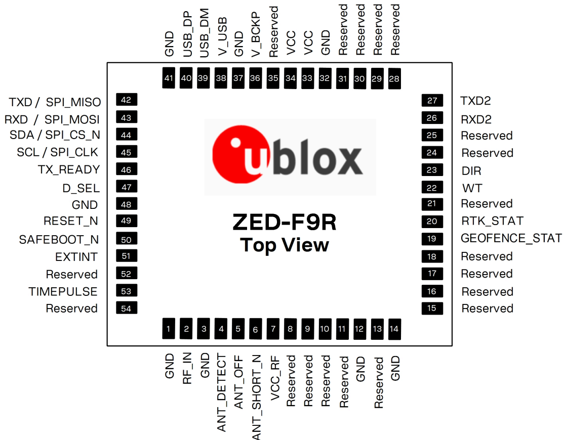
Figure 2: ZED-F9R-02B pin assignment
