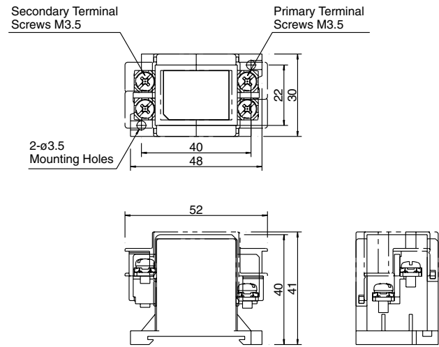
Dimensions (mm)
