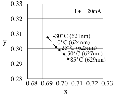
Forward Current vs. Chromaticity Coordinate ( \lambda D )
