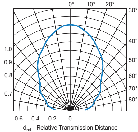
Fig. 11 - Horizontal Directivity
