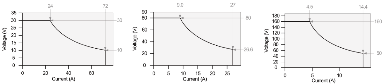
Operating areas of 720 W Models: T3PS30721P, T3PS80271P, T3PS160141P
