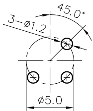
PCB Layout
