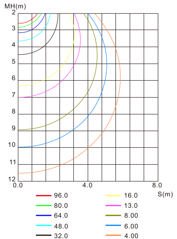
Spacing iso-illuminance curve
