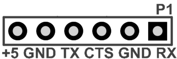
P1 – UART connector P1.1 – RX P1.2 – GND P1.3 – CTS P1.4 – TX P1.5 – GND P1.6 – +5V
