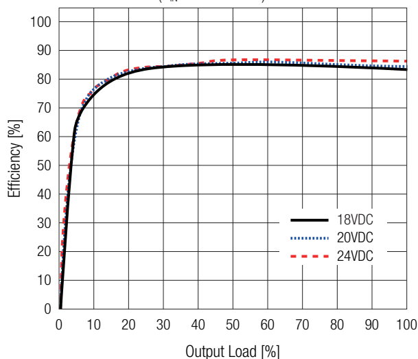
Efficiency vs. Load ( V_{IN}= 18-24VDC )
