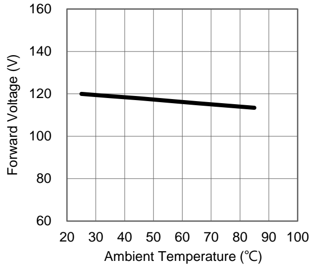
Fig 6. Ambient Temperature vs. Forward Voltage
