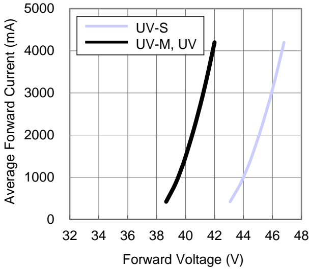
Fig 1. Forward Current vs. Forward Voltage for UV-S, UV-M.
