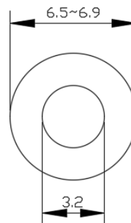
Teflon Washer
