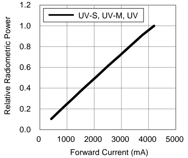
Fig 2. Relative Radiometric Power vs. Forward Current for UV-S, UV-M at T_j=25 maintained.
