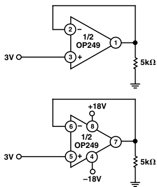
Figure 5. Burn-In Circuit
