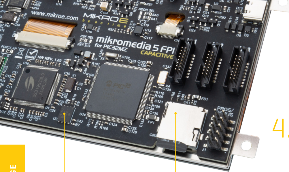
Figure 11: MicroSD card slot view
