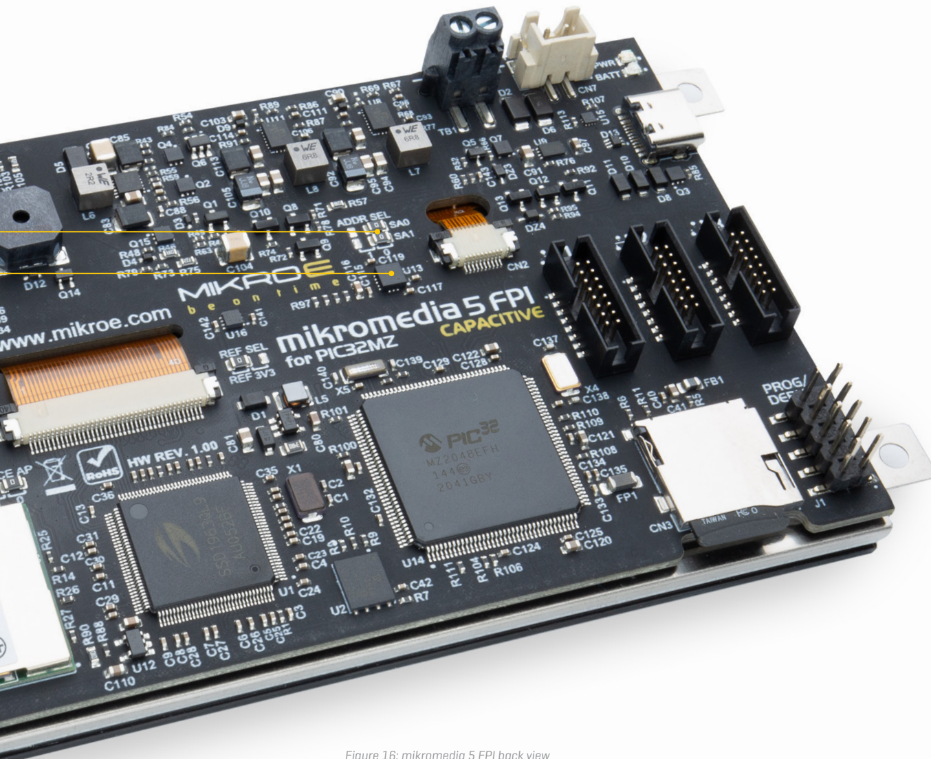
Figure 16: mikromedia 5 FPI back view
