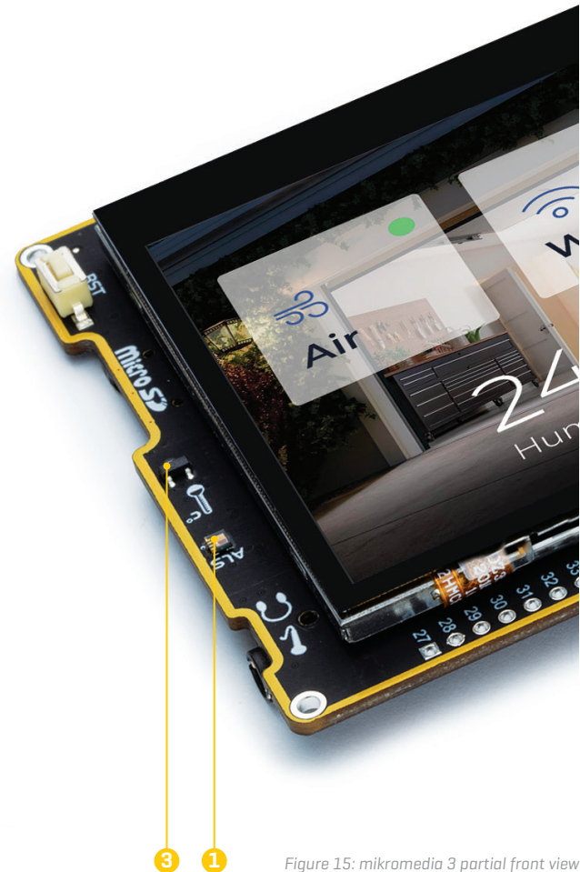
Figure 15: mikromedia 3 partial front view
