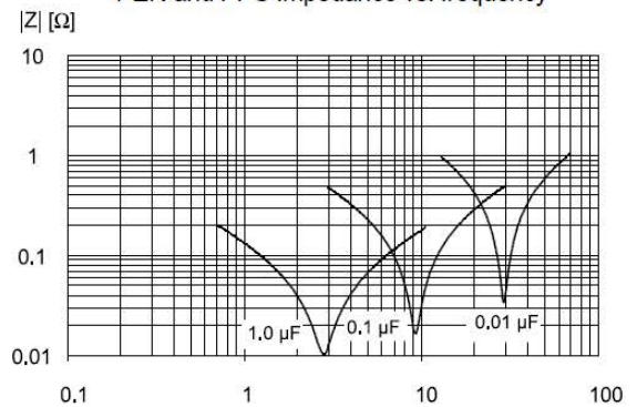
PEN and PPS Impedance vs. frequency
