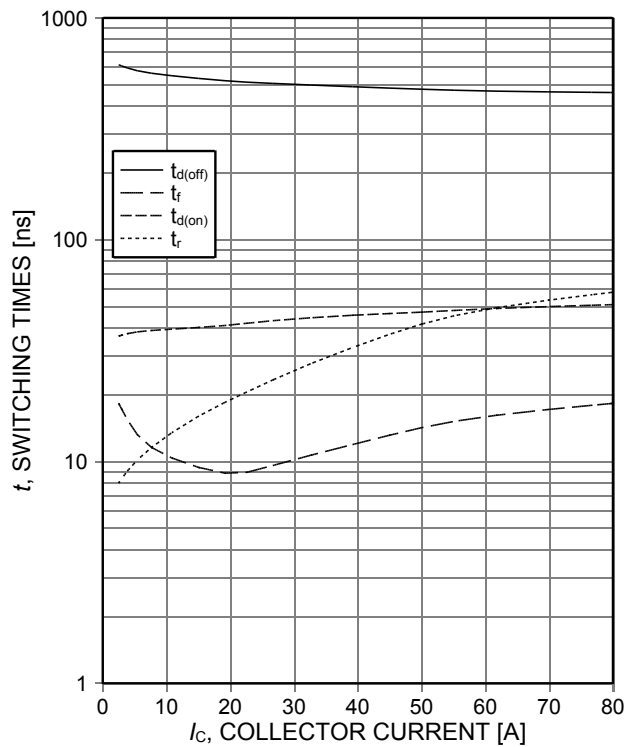
Figure 8. Typical switching times as a function of collector current (inductive load, T_{vj}=175^\circ\text{C} , V_{CE}=400\text{V} , V_{GE}=0/15\text{V} , R_{G(on)}=20\Omega , R_{G(off)}=20\Omega , dynamic test circuit in Figure E)
