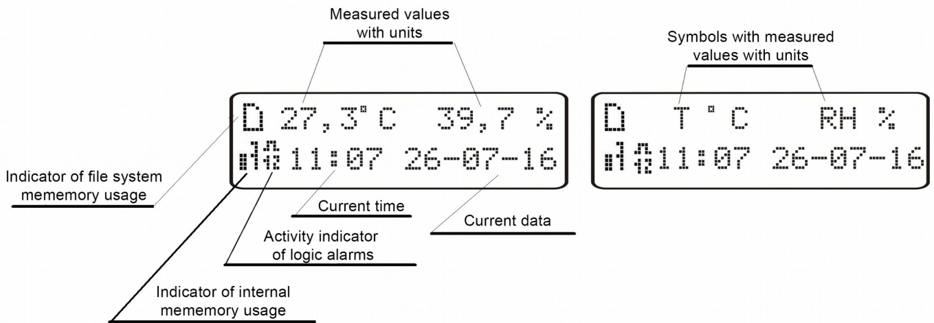
Fig. 5 Description of the HT20IoT monitor reading field
