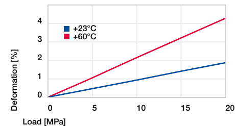
Diagram 03: Deformation under pressure and temperature
