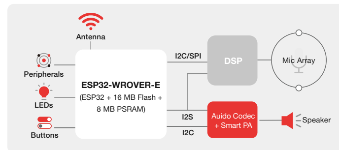
Hardware Architecture
