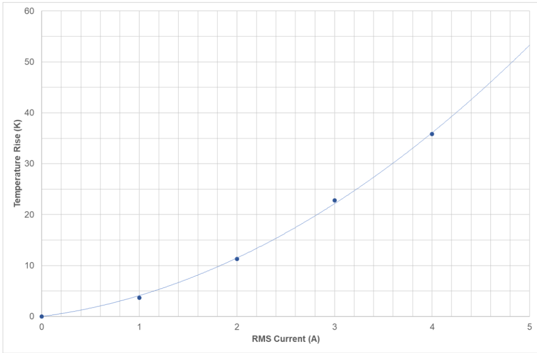
Fig 12: Temperature rise in DMF3Z5R5H474M3DTA0 with RMS current
