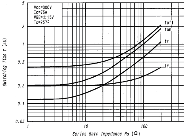
Fig. 7 Series Gate Impedance vs. Switching Time (Typical)
