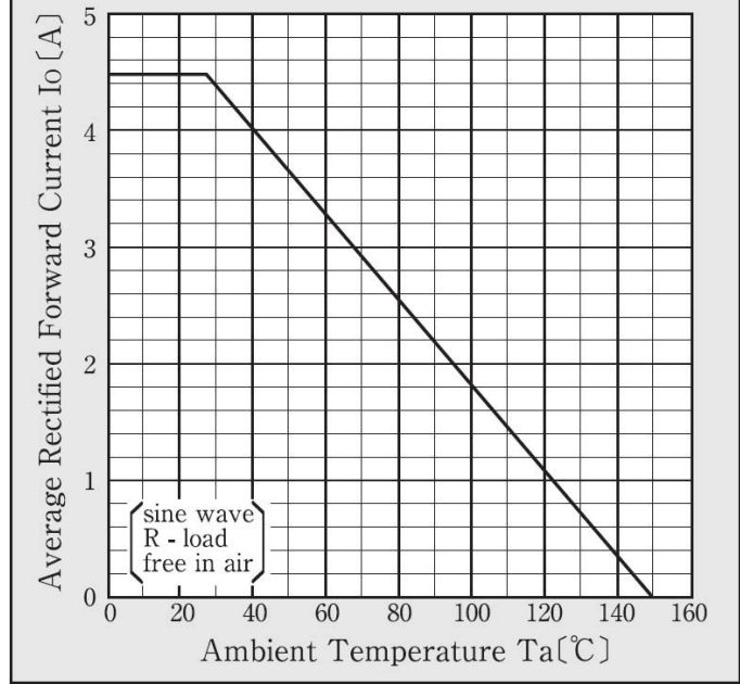
Derating Curve
