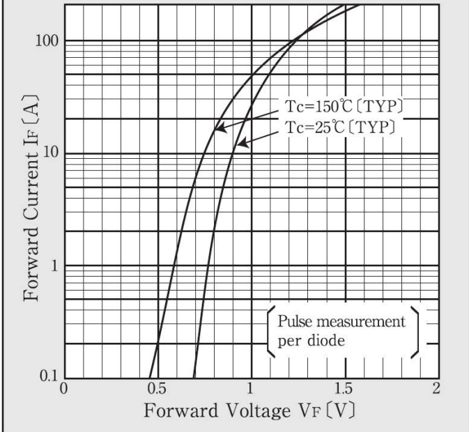
Forward Voltage
