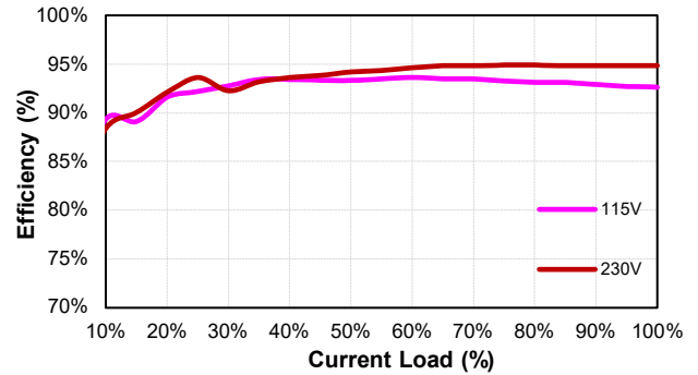
CFM500S360 (Eff Vs Io)
