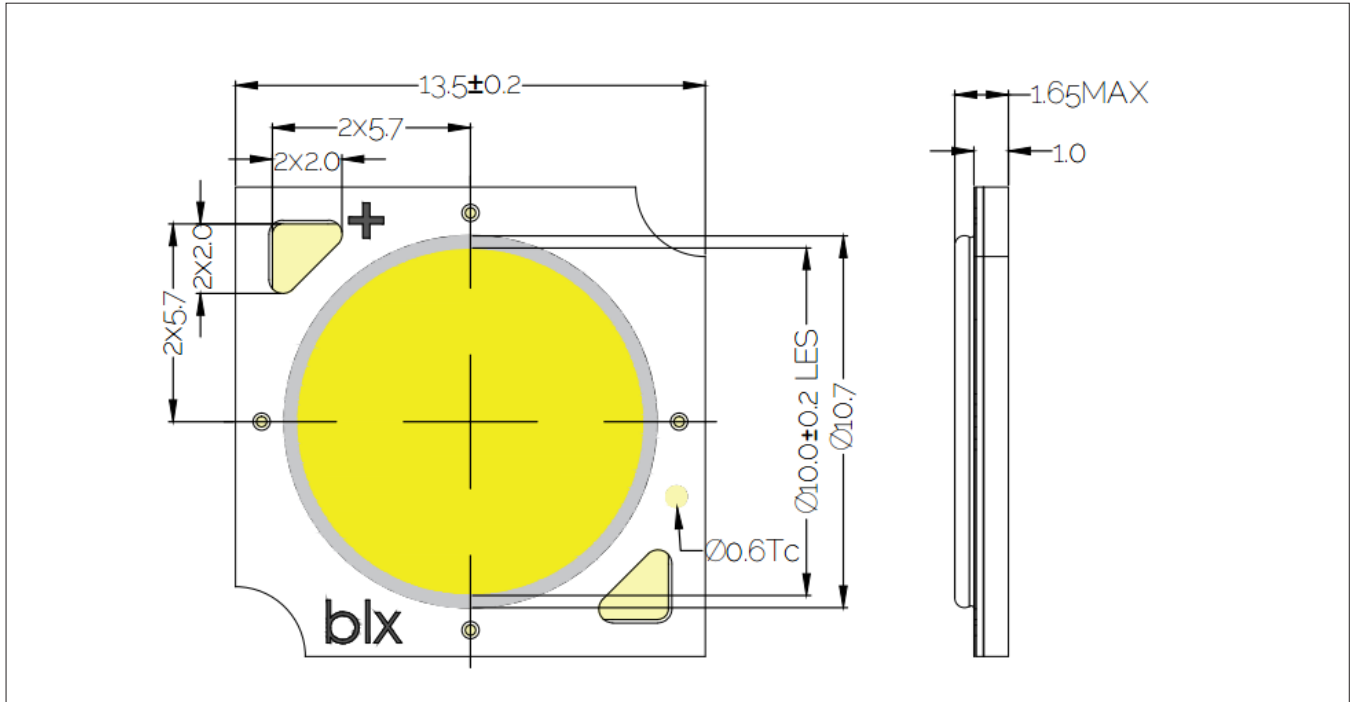
Figure 20: V10 LED Array
