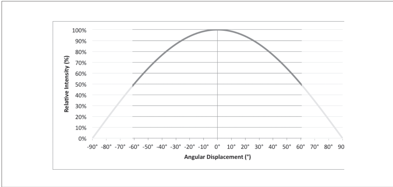
Figure 17: Typical Spatial Radiation Pattern
