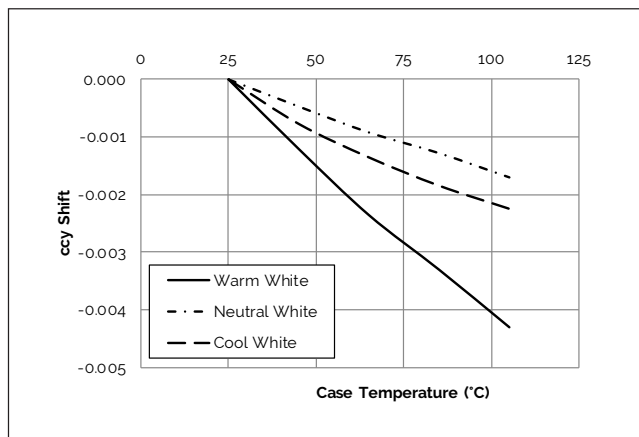
Figure 16: Typical ccy Shift vs. Case Temperature
