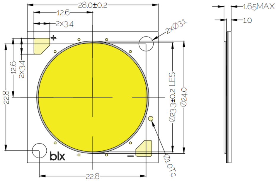
Figure 20: Drawing for V22 LED Array
