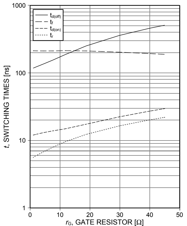
Figure 8. Typical switching times as a function of gate resistor (inductive load, T vj =175°C, V CE =400V, V GE =15/0V, I C =15A, Dynamic test circuit in Figure E)
