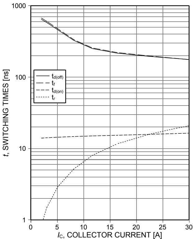
Figure 7. Typical switching times as a function of collector current (inductive load, T vj =175°C, V CE =400V, V GE =15/0V, r G =15Ω, Dynamic test circuit in Figure E)
