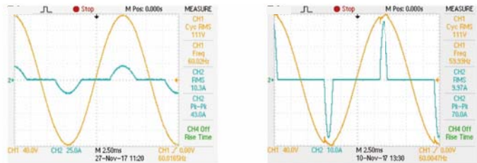
Non-Linear CC mode for UPS test
