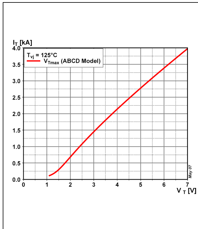
Fig. 3 On-state voltage characteristics 10 ms sine half wave
