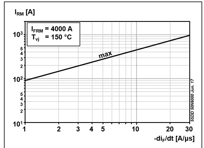
Fig. 7 Peak reverse recovery current vs. decay rate of on-state current
