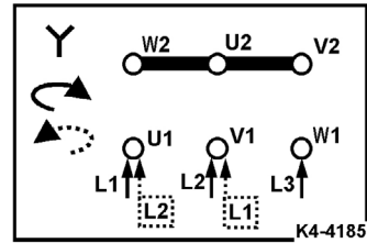
Star connection
