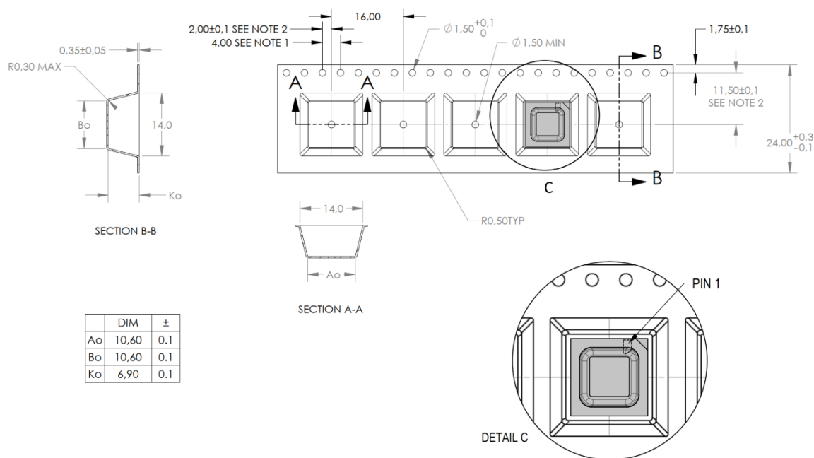
Figure 5: Technical drawing of the packaging tape with sensor orientation in tape. Header tape is to the right and trailer tape to the left on this drawing. Dimensions are given in millimeters.
