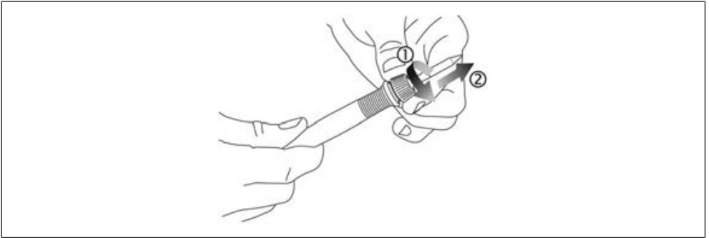
Fig. 1: Unlock [1] and pull out [2] the soldering tip
