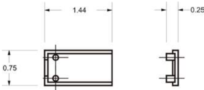
Low Profile Connector Cap
