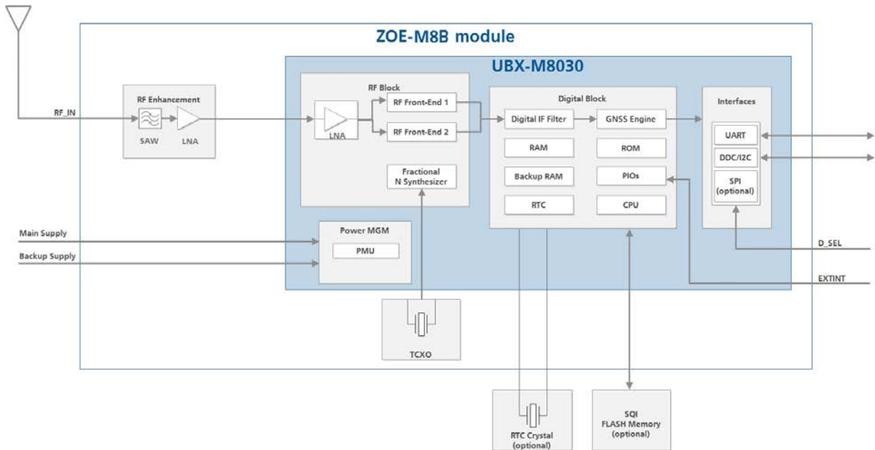
Figure 1: ZOE-M8B block diagram
