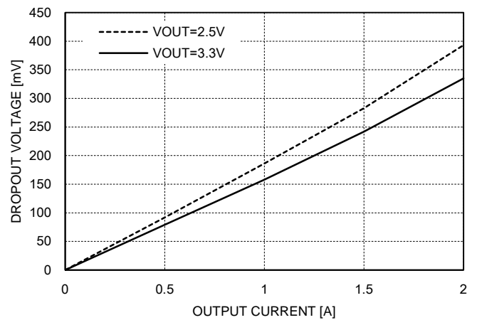
Dropout Voltage
