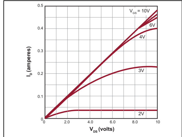
FIGURE 2-4: Saturation Characteristics.
