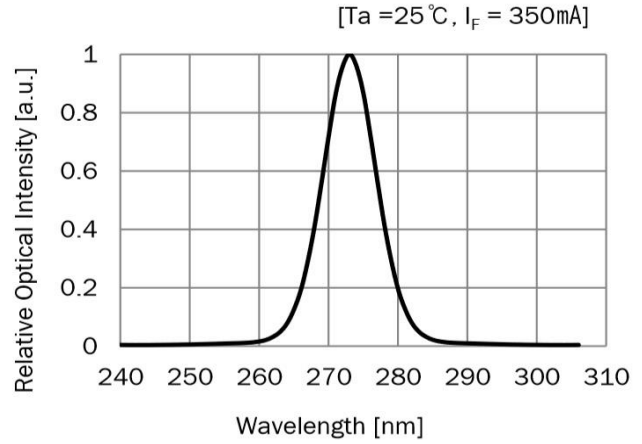
FIG 4. Spectrum
