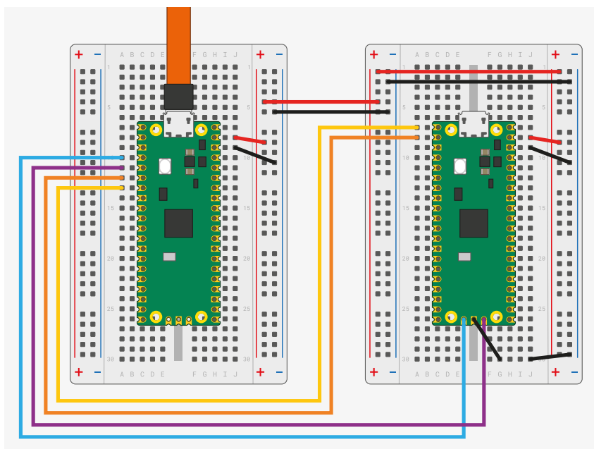
Figure 34. Wiring between PicoA (left) and PicoB (right) configuring Pico A as a debugger. Note that if Pico B is a USB Host then you'd want to hook VBUS up to VBUS so it can provide 5V instead of VSYS to VSYS.
