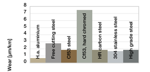
Diagram 06: Wear, rotating with different shaft materials, pressure, p = 1\text{MPa} , v = 0.3\text{m/s}
