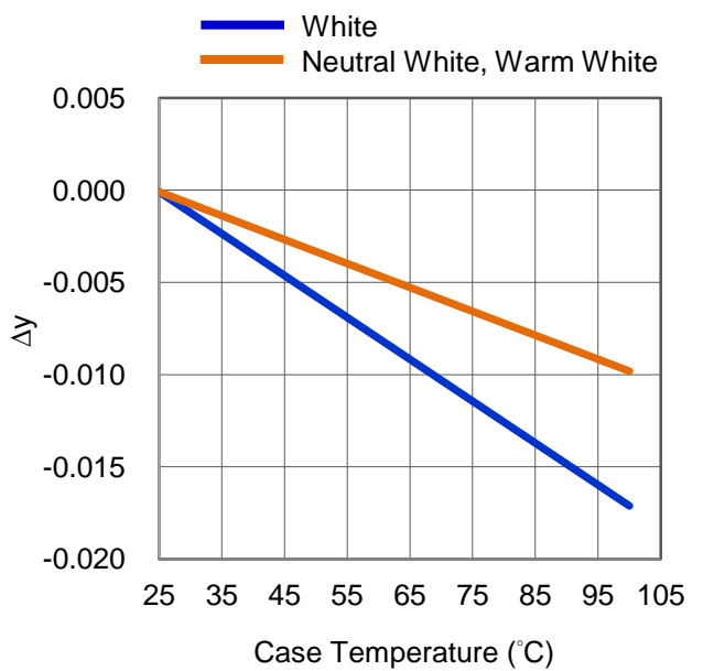
Fig 4. Case Temperature vs. Chromaticity Coordinate \Delta y at 480mA.
