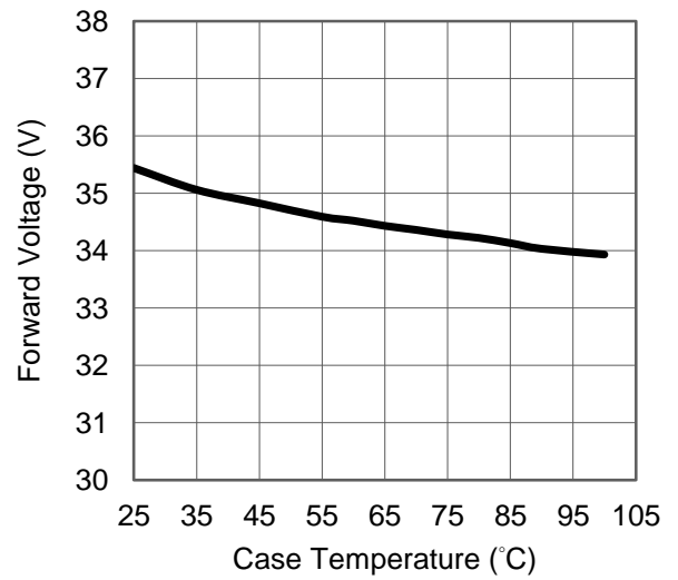
Fig 2. Case Temperature vs. Forward Voltage at 480mA.
