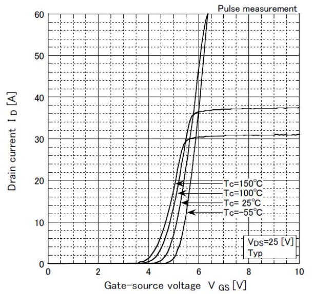
Transfer characteristics
