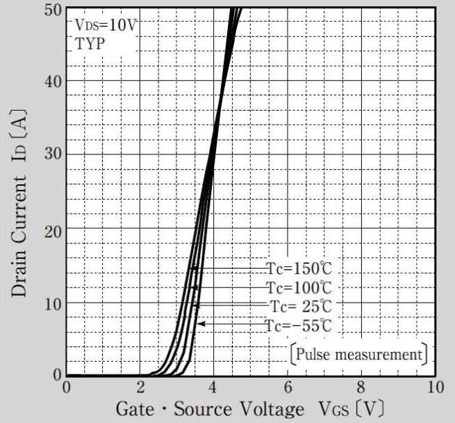
Transfer Characteristics
