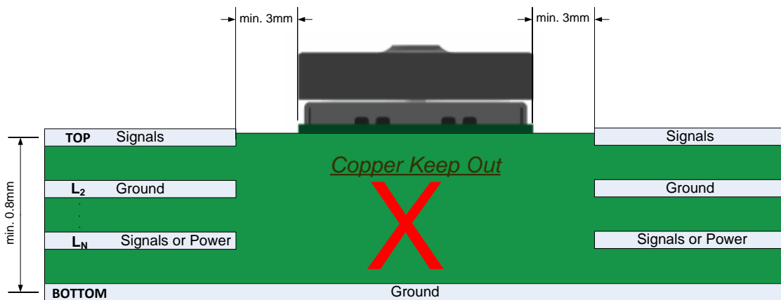
FIGURE 14 – TYPICAL PCB STACK-UP
