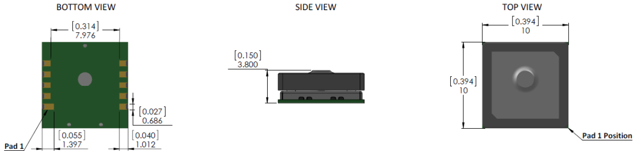
FIGURE 18 – MECHANICAL DRAWING
