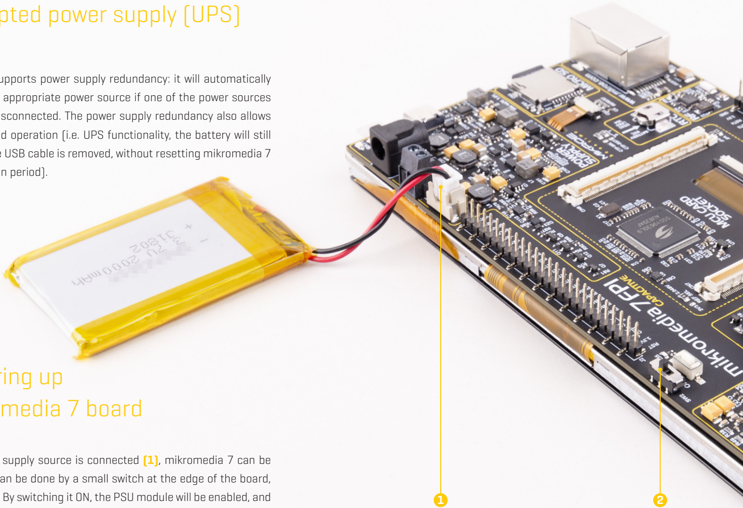
Figure 8: Battery power supply connection view
