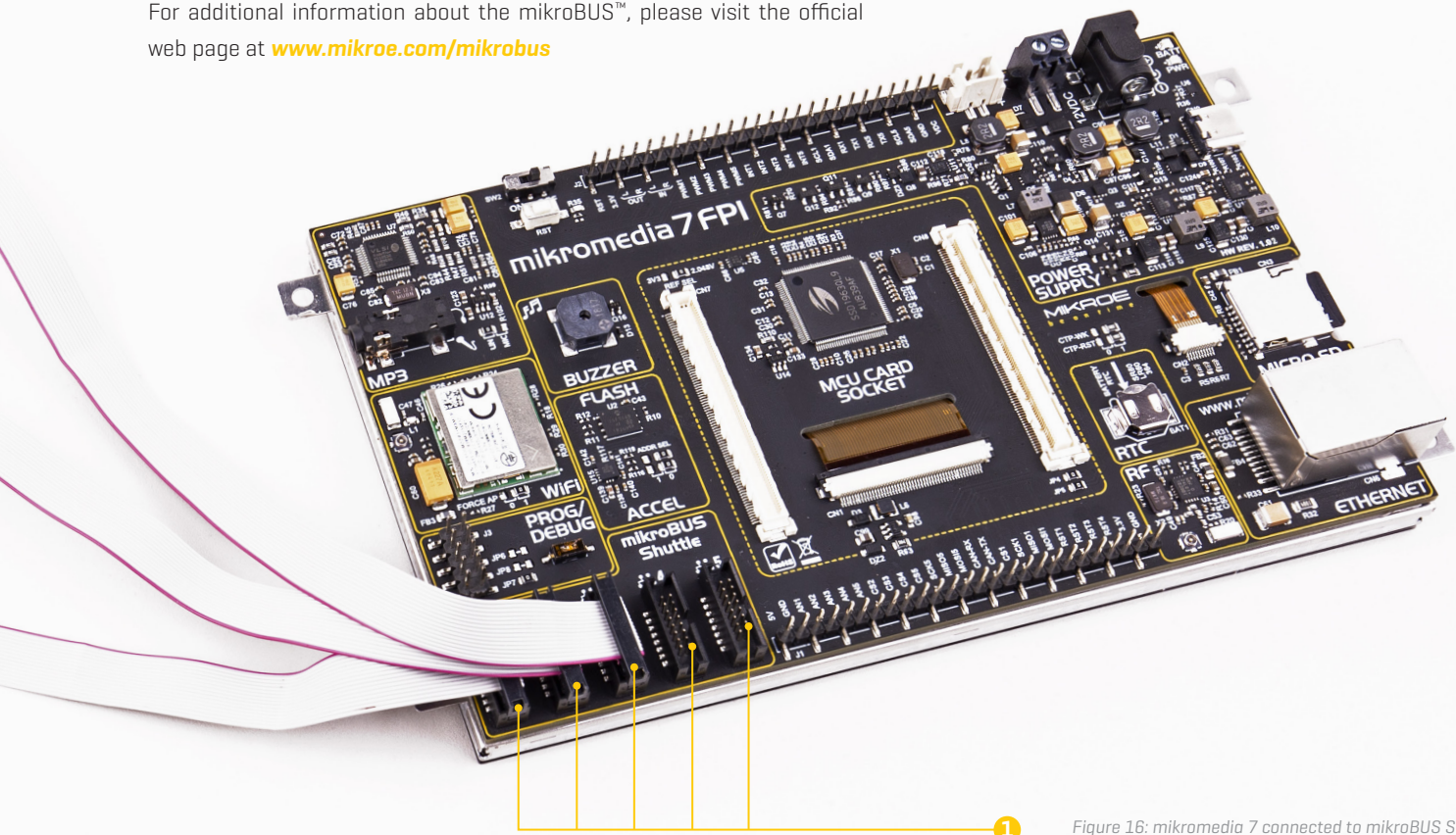
1 Figure 16: mikromedia 7 connected to mikroBUS Shuttle view
