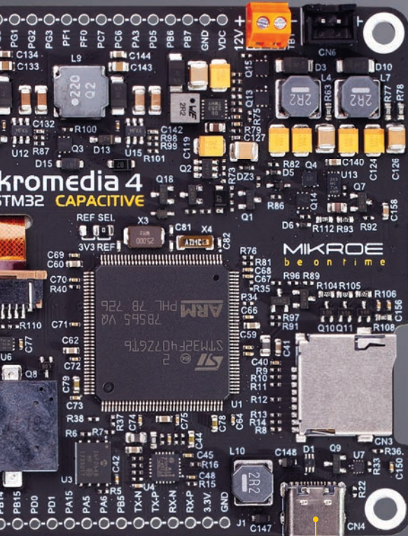
Figure 1.3: mikromedia 4 board – back view
