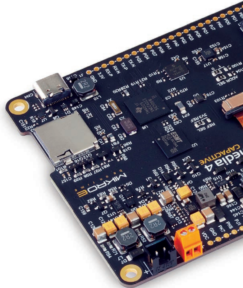
Figure 16: mikromedia 4 back view
