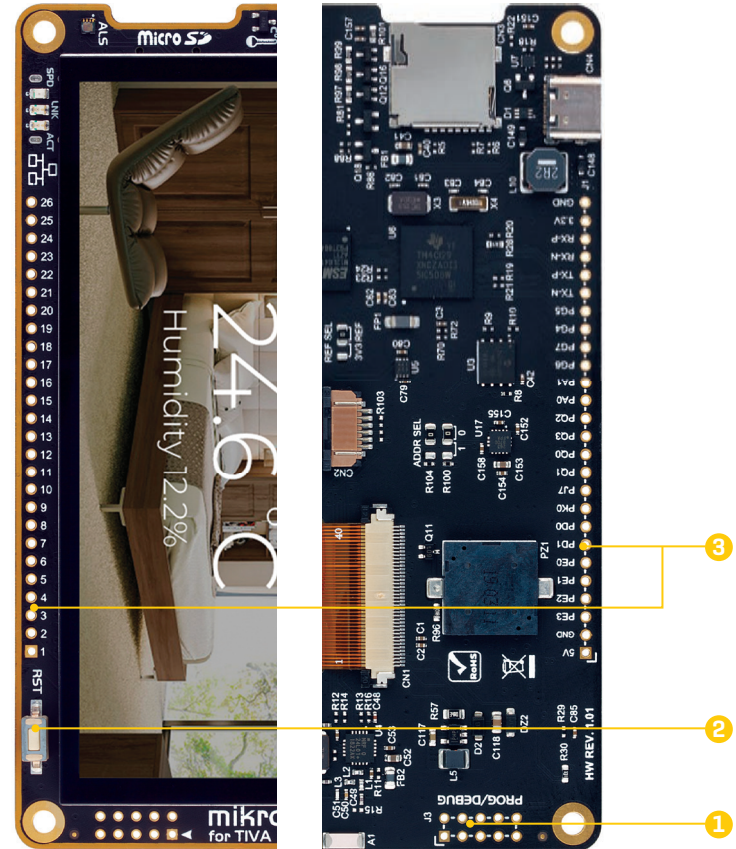
Figure 3: Front and back partial view
