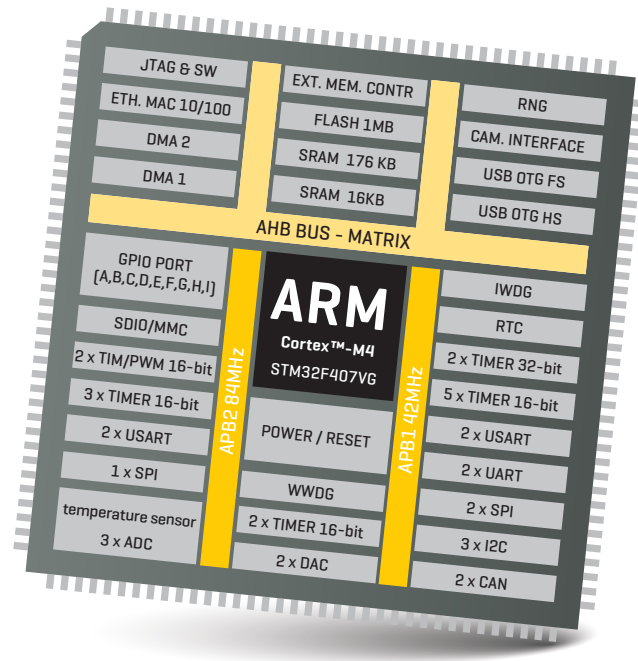
Figure 1: MCU block schematic
