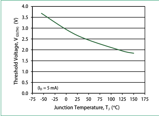
Figure 13: Threshold Voltage
