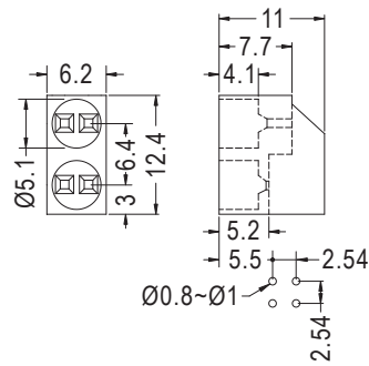
MOUNTING HOLE
