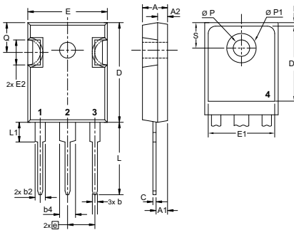
X014a TO-247 AD Weight = 6 g
