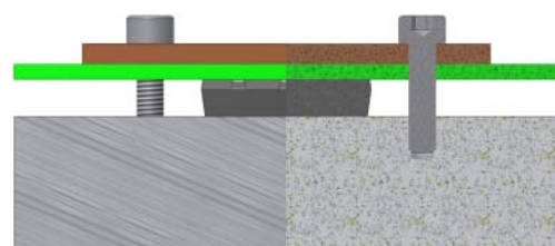
Fig. 4 Mounting example
