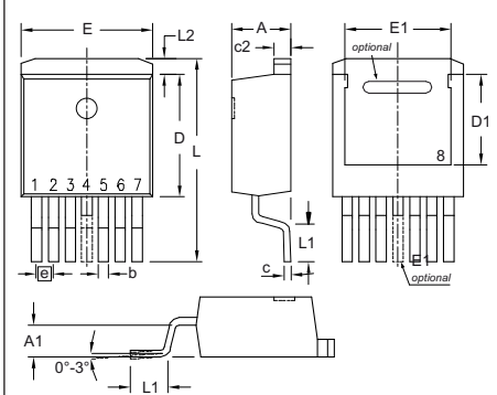
X012b TO-263 (7) c) middle leg cut Weight = 2.5 g
